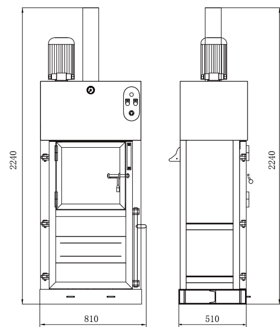
Diagram (Model SX-100LA6040)
