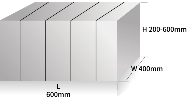
Bale Size (Model SX-100LA6040)
