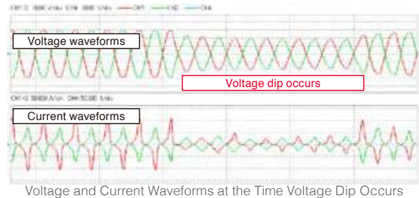
Voltage and Current Waveforms at the Time Voltage Dip Occurs
