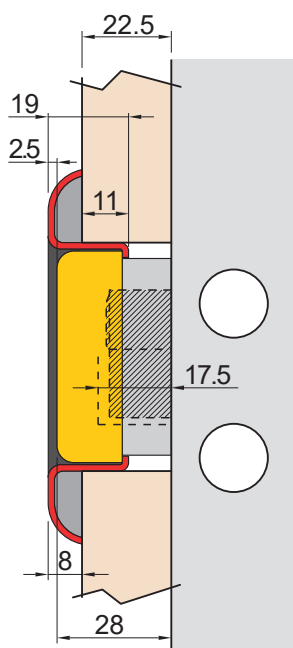
KM0P96 CHIAVE MAGNETICA MAGNETIC KEY
