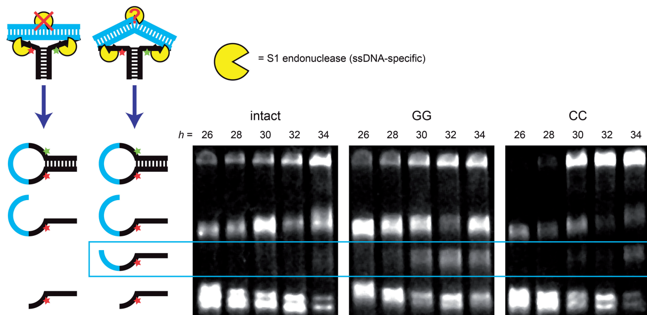
Figure 4. Cleavage of kinked target strands in a molecular vise by S1 endonuclease at high ionic strength. Molecular vises with a 36-nt loop and varying length target strands were treated with the single-stranded DNA-specific S1 nuclease in a high-ionic-strength buffer and analyzed by denaturing PAGE. The target strands were either fully complementary (left image) or contained a single GG (center image) or CC (right image) mismatch. The different complexes reacted at different rates; the cleavage reactions were quenched at 135 min (intact, left), 15 min (GG, center) or 45 min (CC, right). Cartoons on the left depict cleavage products and reactants. The longest band (top) was the undigested hairpin. Of the cleavage products, the longest resulted from cleavage of the loop at its 3' end; the shortest resulted from cleavage of the loop at its 5' end; and the middle band, when present, resulted from cleavage within the target strand. This band appeared weakly in the intact target strand of length 34 bp, and prominently in the mismatched target strands of length >30 bp. Cleavage within the target strand indicated kinking-induced disruption of base pairing.
