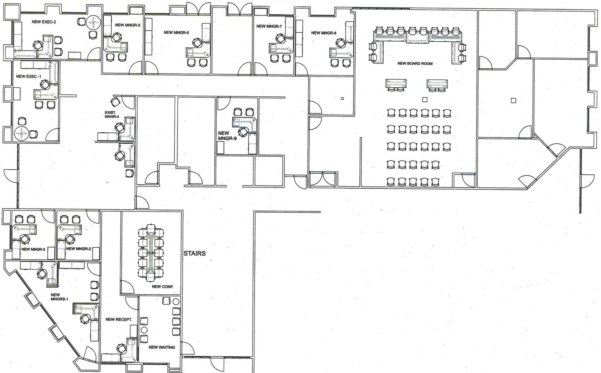
FLOOR PLAN
