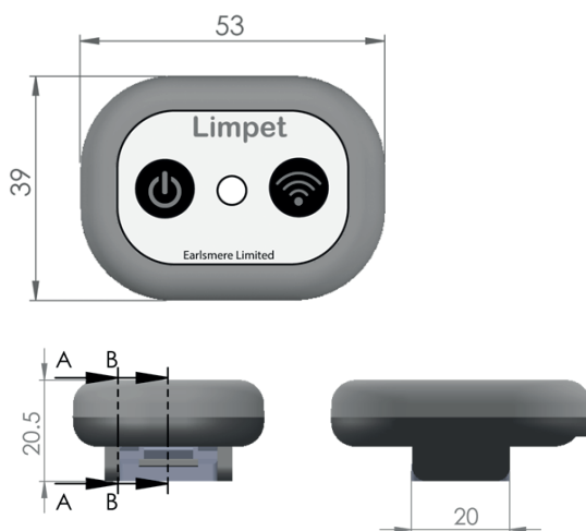
Limpet Dimensions (mm)
