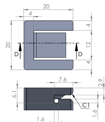
Limpet Holder Dimensions (mm)
