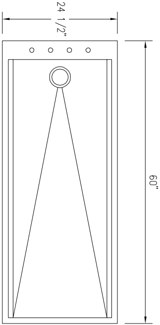
PLAN VIEW
