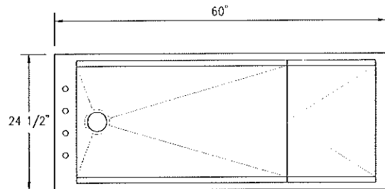
PLAN VIEW
