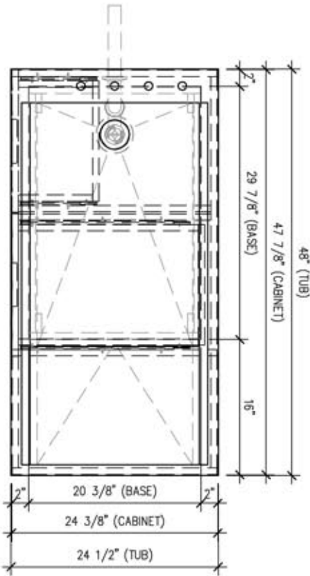
PLAN VIEW NOT TO SCALE
