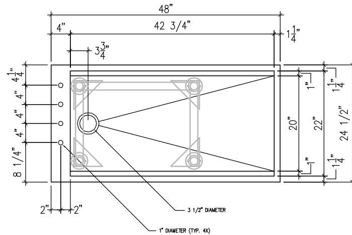
PLAN VIEW SCALE: 2" = 1'-0"
