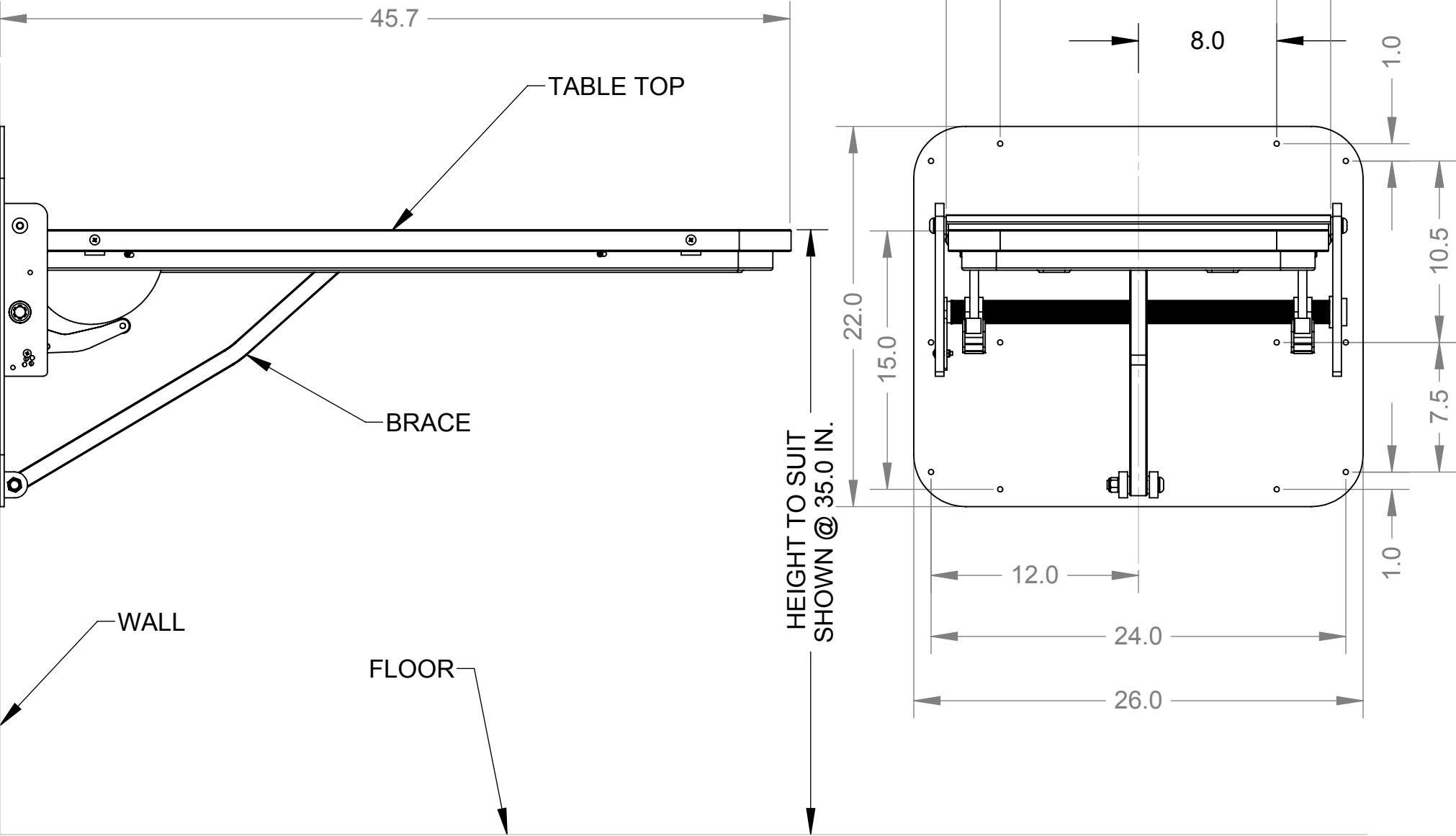
MOUNTING DETAIL FOLD UP WALL MOUNT EXAM TABLE
