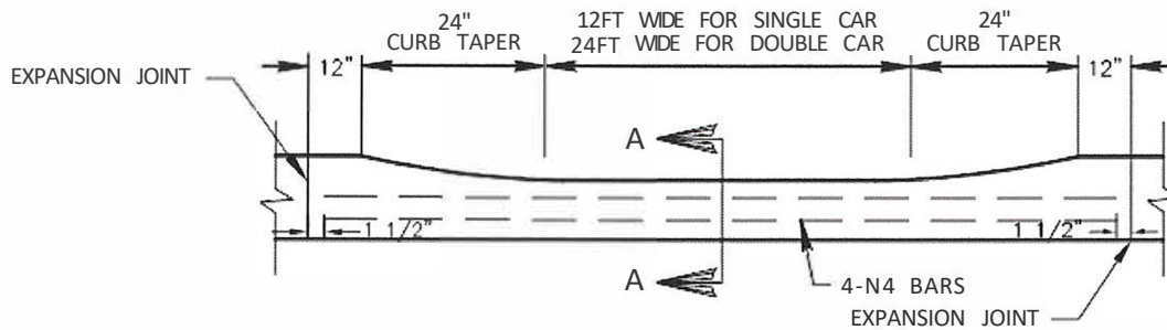
PLAN VIEW
