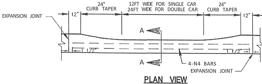
Depressed Concrete Curb Detail (Not to Scale)
