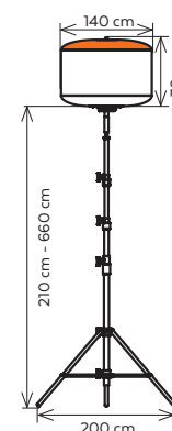
P600TA stand
