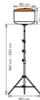
P500TA stand
