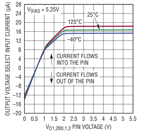
V_{O1,2B0,1,2} Pin Input Current
