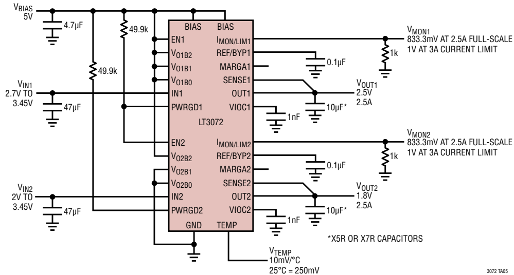
BIAS/2.5V/1.8V Supply Sequencing
