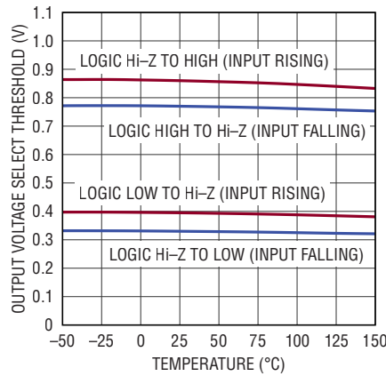
V_{O1,2B0,1,2} Pin Thresholds
