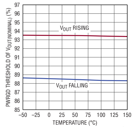
PWRGD Threshold
