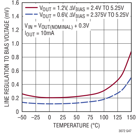
Line Regulation to V_{BIAS}
