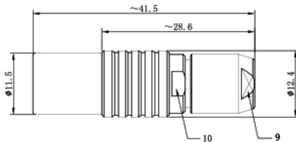
CONNECTOR SOLDER CUP VIEW
