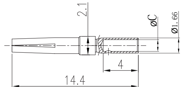
Crimp Contact, Female
