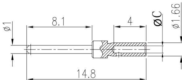
Crimp Contact, Male
