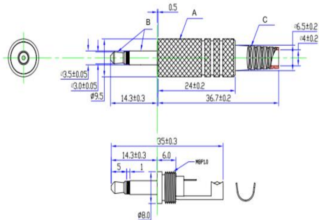
Dimensions: (mm)
