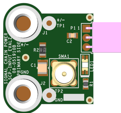
Figure 1. SCP-INPUT-EVALZ Board
