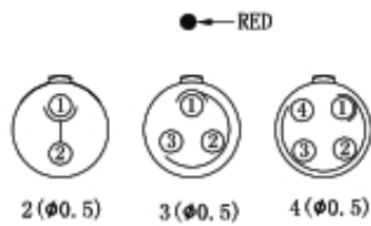
CONNECTOR SOLDER CUP VIEW
