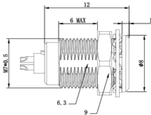
CONNECTOR SOLDER CUP VIEW
