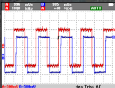
500 MHz bandwidth and 5GS/s sampling can reveal signal noise and distortion that otherwise may go undetected.
