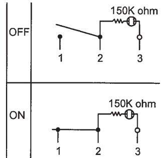
Circuit Diagram
