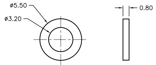
WASHER (2PCS)
