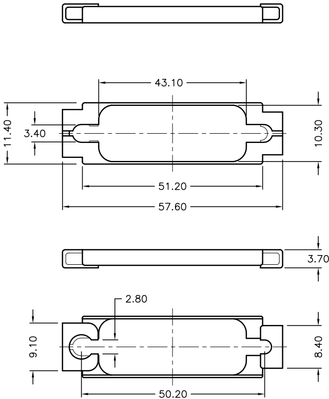
SLIDE LATCH
