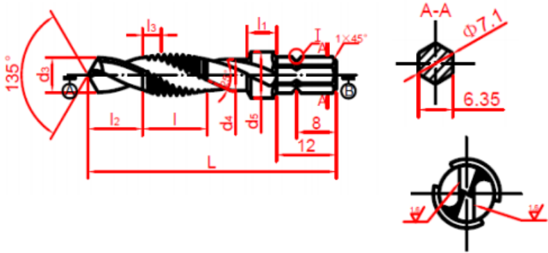
1/4in hexagon 6pcs drive drilltap
