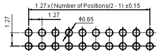
PCB Layout
