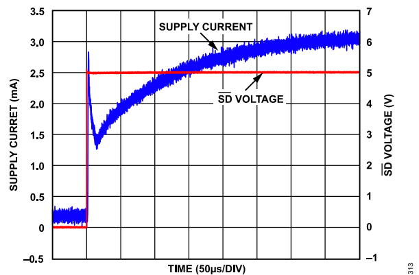
Figure 53. \overline{SD} Pin Response Time, Turning On
