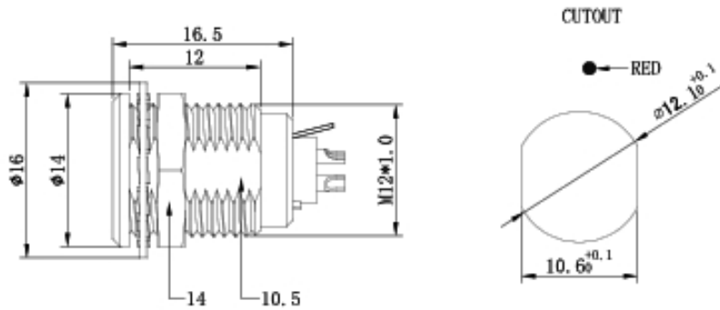
CONNECTOR SOLDER CUP VIEW
