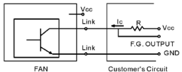
Tachometer - Open Collector
