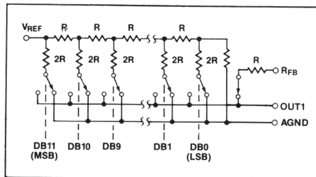
Figure 1. Simplified D/A Circuit of MX7548
