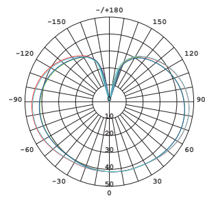
A60F8-D-8.5W-E-E27
