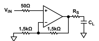
Figure 69. Circuit for Capacitive Load Drive
