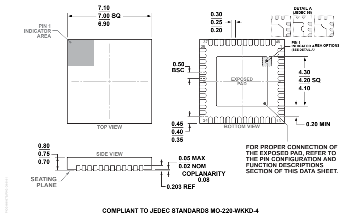
Figure 81. 48-Lead Dual-Pad Lead Frame Chip Scale Package [LFCSP] 7 mm x 7 mm Body and 0.75 mm Package Height (CP-48-17) Dimensions shown in millimeters
