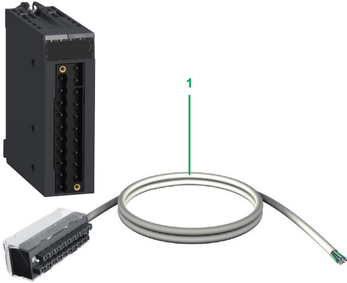
BMXFTW01S cordset (with 20-way removable terminal block at one end and flying leads at the other)
