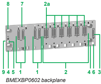
BMEXBP0602 backplane
