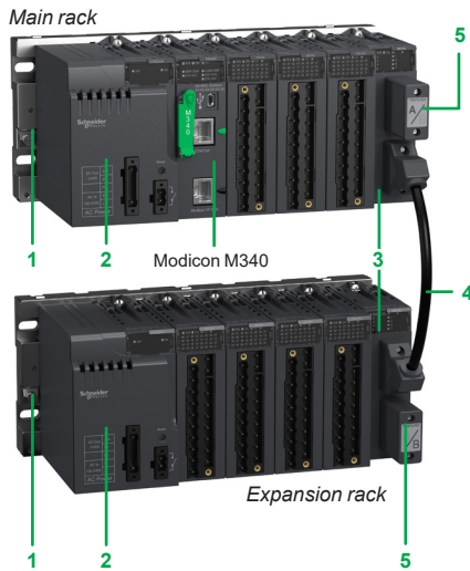
Station with Modicon M340 in main rack + expansion rack
