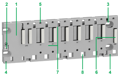
BMXXBP0600 backplane with 6 slots
