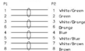
PIN ASSIGNMENT (TIA 568A)
