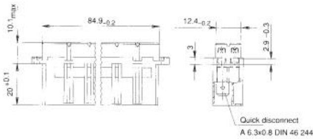
Female connector with quick disconnect termination
