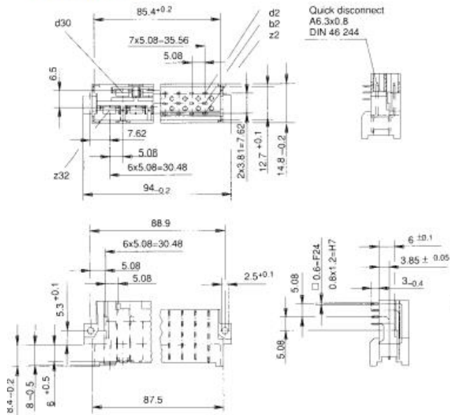
Male connector
