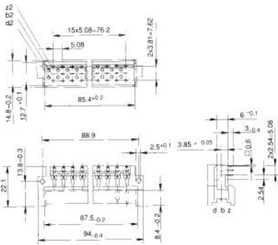
Male connector
