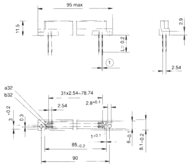
Female connector
