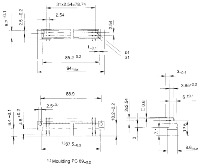
Male connector
