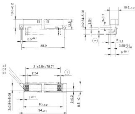
Female connector
