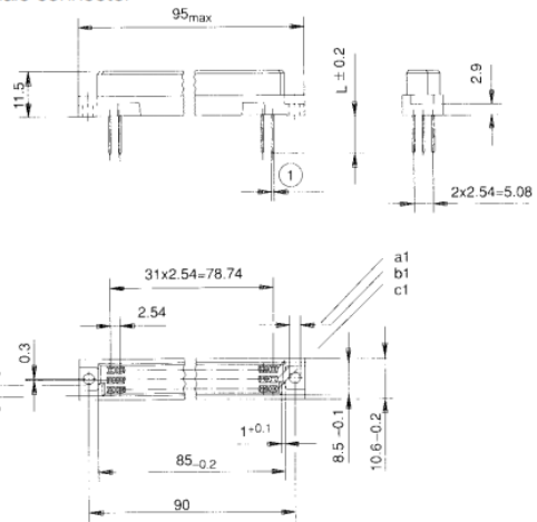
Female connector
