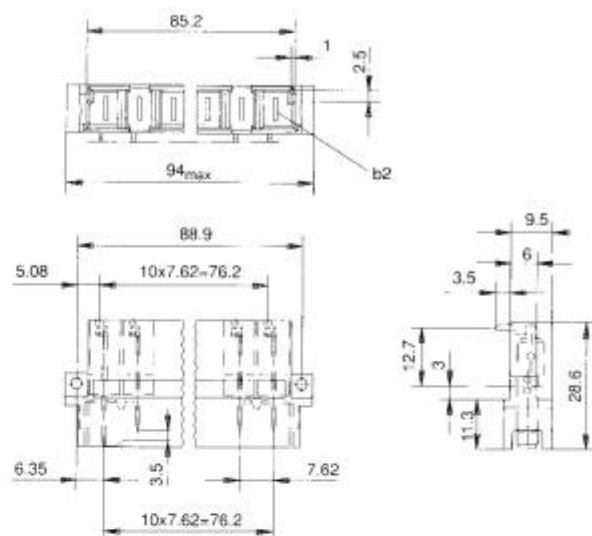
Male connector
