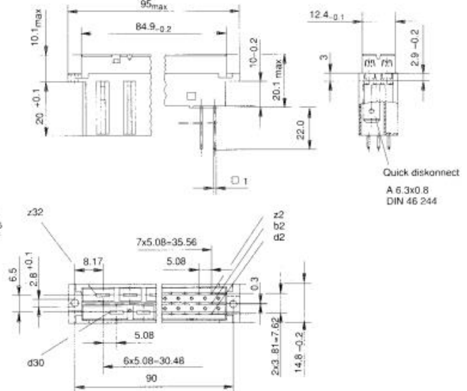
Female connector
