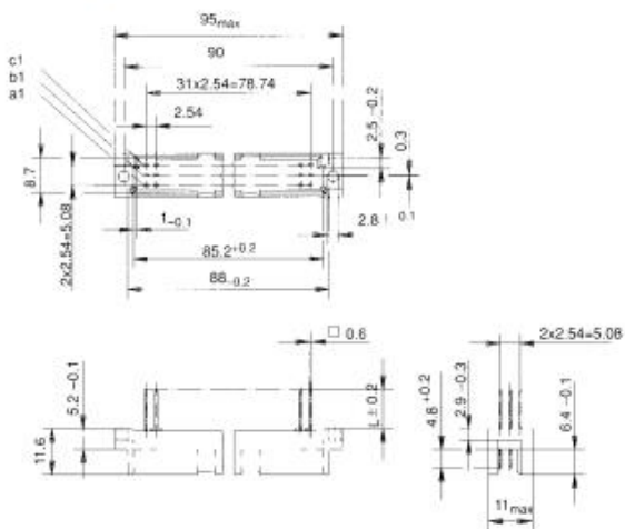
Male connector
