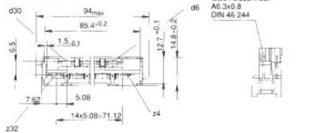
Male connector
