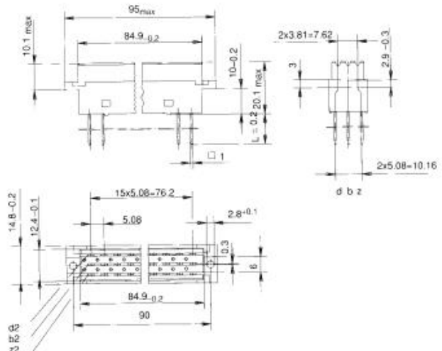
Female connector
