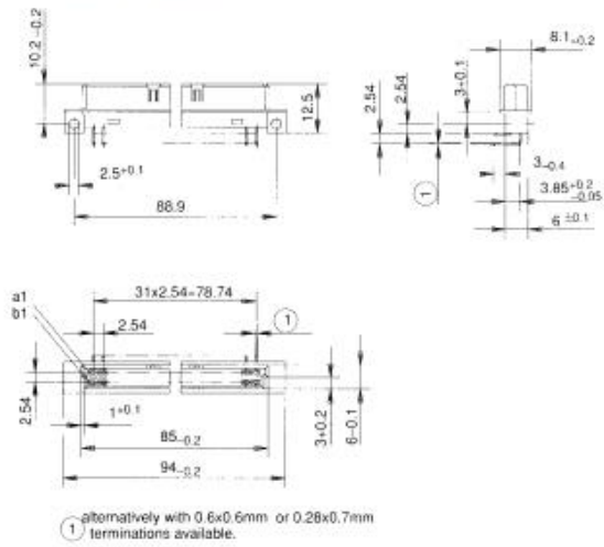
Female connector
