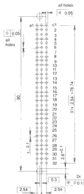
Hole pattern 1
