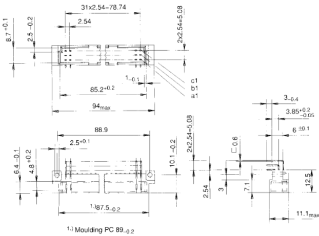
Male connector
