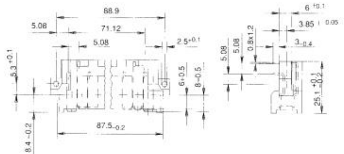
Female connector with dip solder termination
