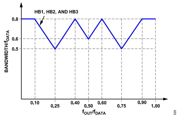
Figure 59. Signal Bandwidth vs. Center Frequency of the Output Signal, 8x Interpolation
