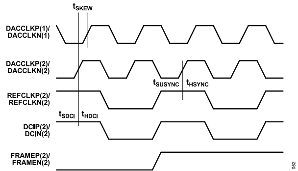
Figure 84. Data Rate Synchronization Signal Timing Requirements, 2× Interpolation
