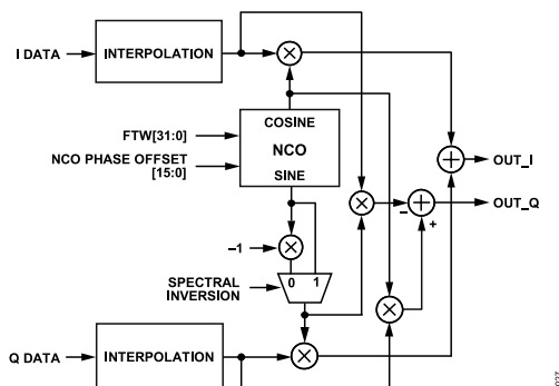
Figure 57. Digital Quadrature Modulator Block Diagram
