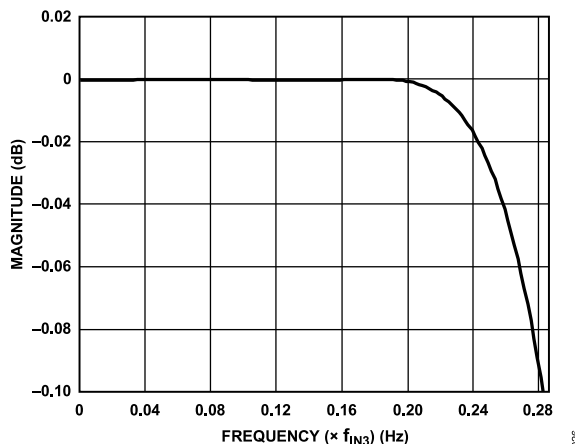
Figure 56. Pass-Band Detail of HB3
