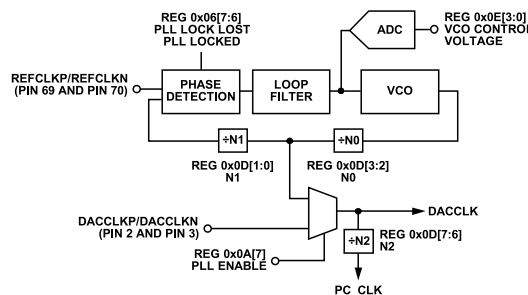
Figure 64. PLL Clock Multiplication Circuit
