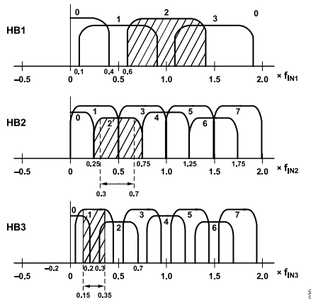
Figure 60. Signal Propagation for 8× Interpolation ( f_{DATA} Modulation)
