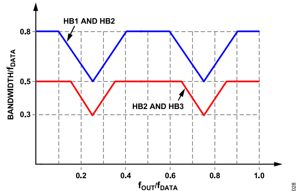
Figure 58. Signal Bandwidth vs. Center Frequency of the Output Signal, 4x Interpolation
