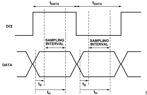
Figure 46. Timing Diagram for Input Data Port
