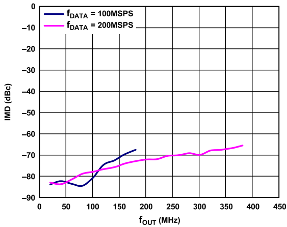
Figure 17. IMD vs. f_{OUT} over f_{DATA} , 4× Interpolation, Digital Scale = 0 dBFS, I_{FS} = 20\text{ mA}
