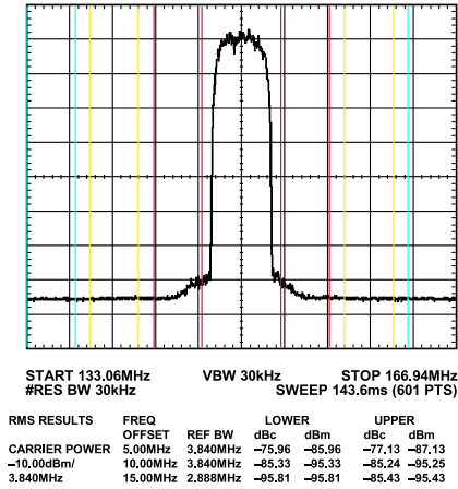
Figure 34. One-Carrier W-CDMA ACLR Performance, IF = ~150 MHz
