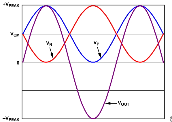
Figure 69. Output Voltage Waveforms
