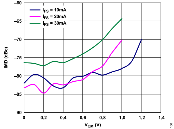
Figure 70. IMD vs. Output Common-Mode Voltage ( f_{OUT} = 61 \text{ MHz} , R_{LOAD} = 50 \Omega Differential, I_{FS} = 10 \text{ mA} , 20 \text{ mA} , and 30 \text{ mA} )
