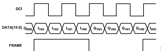
Figure 45. Timing Diagram for Nibble Mode
