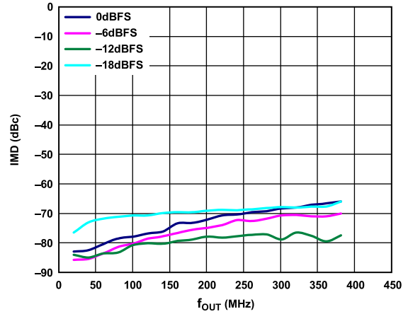
Figure 19. IMD vs. f_{OUT} over Digital Scale, 2× Interpolation, f_{DATA} = 400\text{ MSPS} , I_{FS} = 20\text{ mA}
