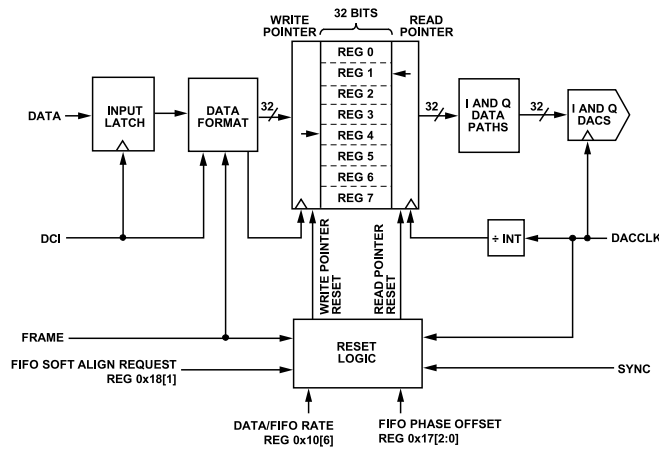
Figure 47. Block Diagram of FIFO
