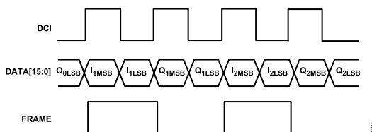
Figure 44. Timing Diagram for Byte Mode
