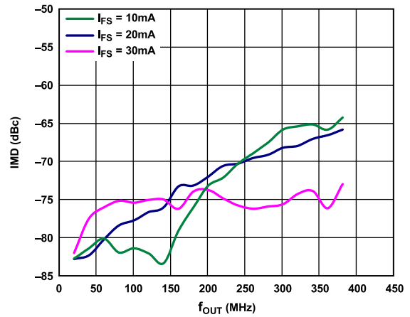
Figure 20. IMD vs. f_{OUT} over I_{FS} , 2× Interpolation, f_{DATA} = 400\text{ MSPS} , Digital Scale = 0 dBFS
