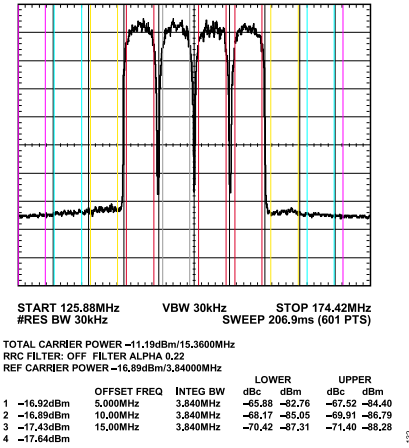
Figure 35. Four-Carrier W-CDMA ACLR Performance, IF = ~150 MHz
