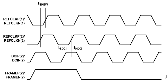
Figure 82. Timing Diagram Required for Synchronizing Devices
