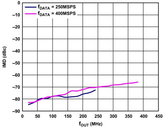
Figure 16. IMD vs. f_{OUT} over f_{DATA} , 2× Interpolation, Digital Scale = 0 dBFS, I_{FS} = 20\text{ mA}
