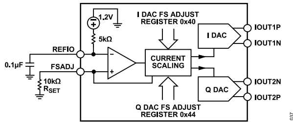
Figure 66. Simplified Block Diagram of DAC Core
