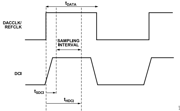
Figure 85. Timing Diagram for Input Data Port (Data Rate Mode)
