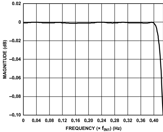
Figure 52. Pass-Band Detail of HB1
