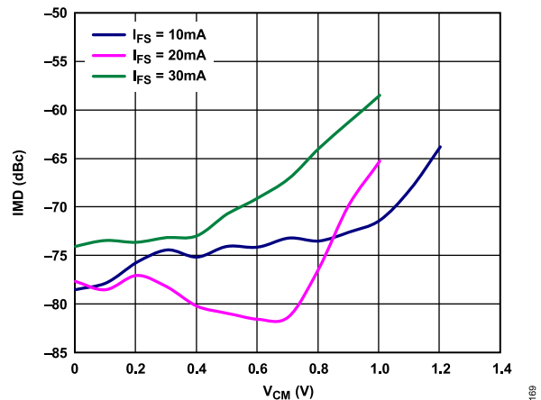
Figure 71. IMD vs. Output Common-Mode Voltage ( f_{OUT} = 161 \text{ MHz} , R_{LOAD} = 50 \Omega Differential, I_{FS} = 10 \text{ mA} , 20 \text{ mA} , and 30 \text{ mA} )
