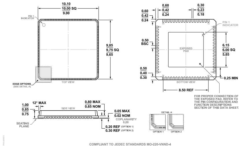
Figure 89. 72-Lead Lead Frame Chip Scale Package [LFCSP] 10 mm × 10 mm Body and 0.85 mm Package Height (CP-72-7) Dimensions shown in millimeters
