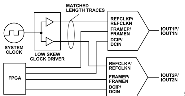
Figure 81. Typical Circuit Diagram for Synchronizing Devices
