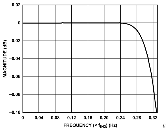
Figure 55. Pass-Band Detail of HB2
