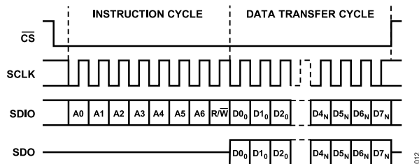
Figure 40. Serial Port Interface Timing, LSB First
