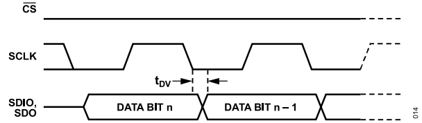
Figure 42. Timing Diagram for Serial Port Register Read.
