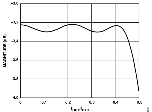
Figure 62. Sample Composite Responses of the Sinc -1 Filter with sin(x)/x Roll-Off
