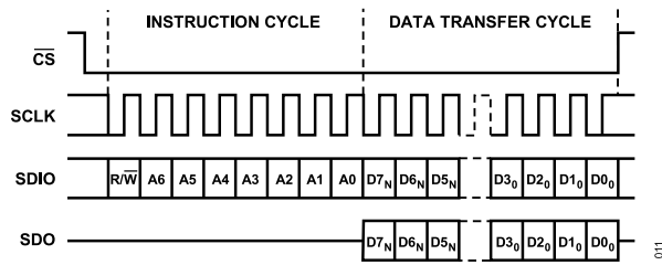
Figure 39. Serial Port Interface Timing, MSB First
