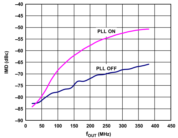
Figure 21. IMD vs. f_{OUT} , 4× Interpolation, f_{DATA} = 200\text{ MSPS} , Digital Scale = 0 dBFS, I_{FS} = 20\text{ mA} , PLL On and PLL Off
