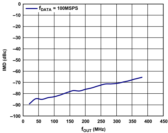
Figure 18. IMD vs. f_{OUT} , 8× Interpolation, f_{DATA} = 100\text{ MSPS} , Digital Scale = 0 dBFS, I_{FS} = 20\text{ mA}
