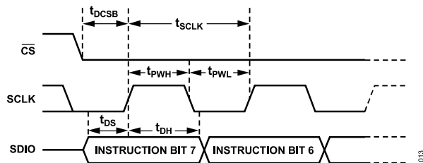
Figure 41. Timing Diagram for Serial Port Register Write
