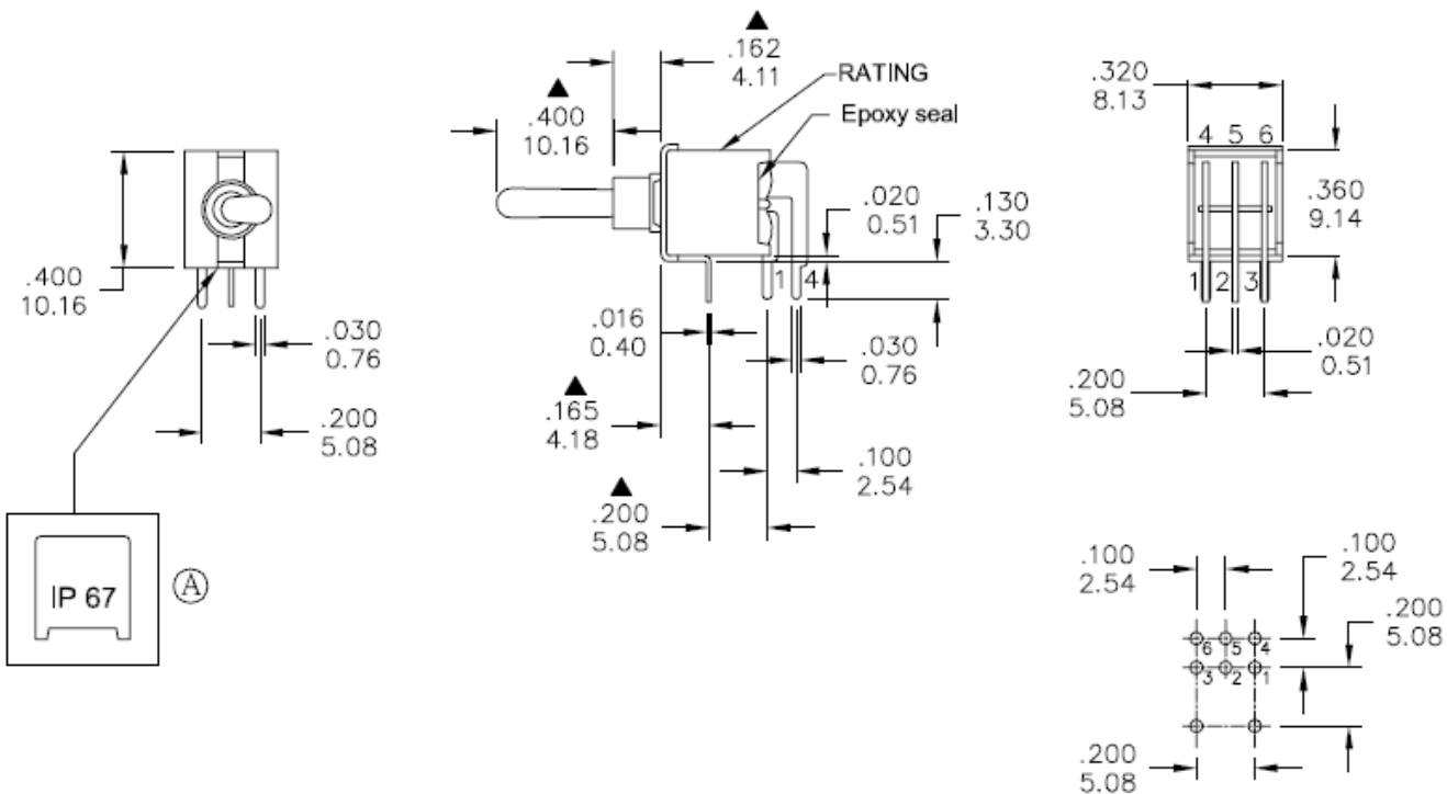
P.C. MOUNTING
