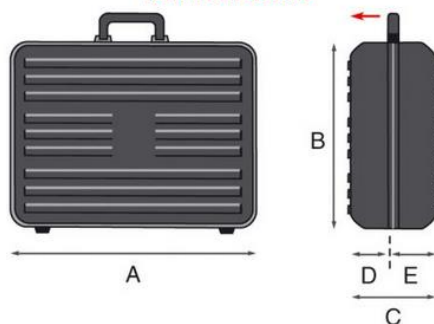
Internal dimensions
