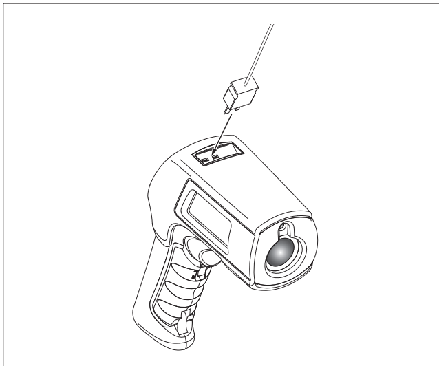
Figure 7. Thermocouple Connection
