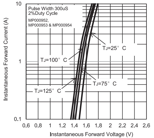
Fig. 6 - Typical Forward Characteristics
