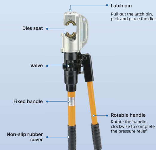
2 2 stage hydraulics, automatic pressure release
