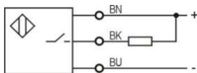
NPN NO
