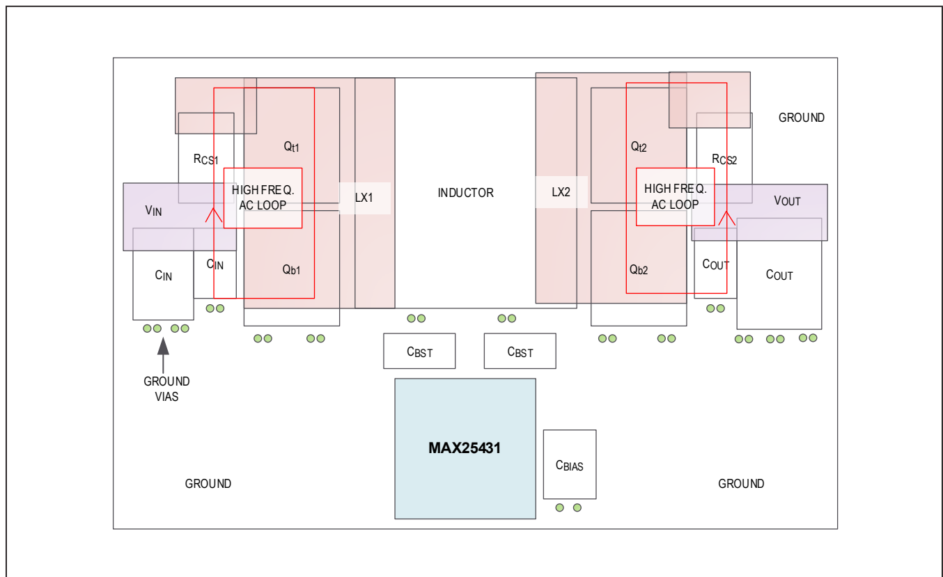
Figure 3. Recommended PCB Layout for the MAX25431.
