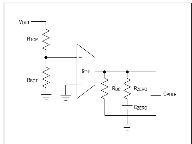
Figure 2. Setting the Output Voltage for the MAX25431.
