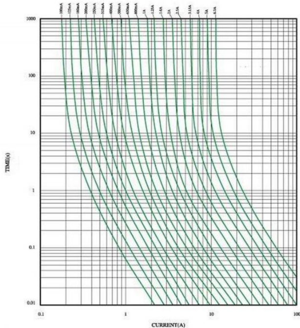
5RT RoHS I-T CHARACTERISTICS CURVE 5RT RoHS
