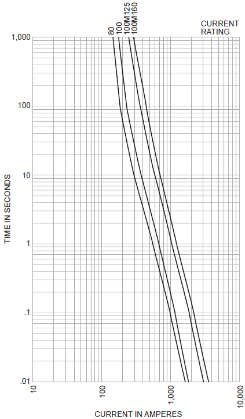
Time-Current Characteristic Curve (Full Size Curves Available)
