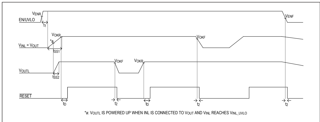
Figure 1. \overline{RESET} Output Logic Diagram when INL is Connected to the Step-Down Converter Output
