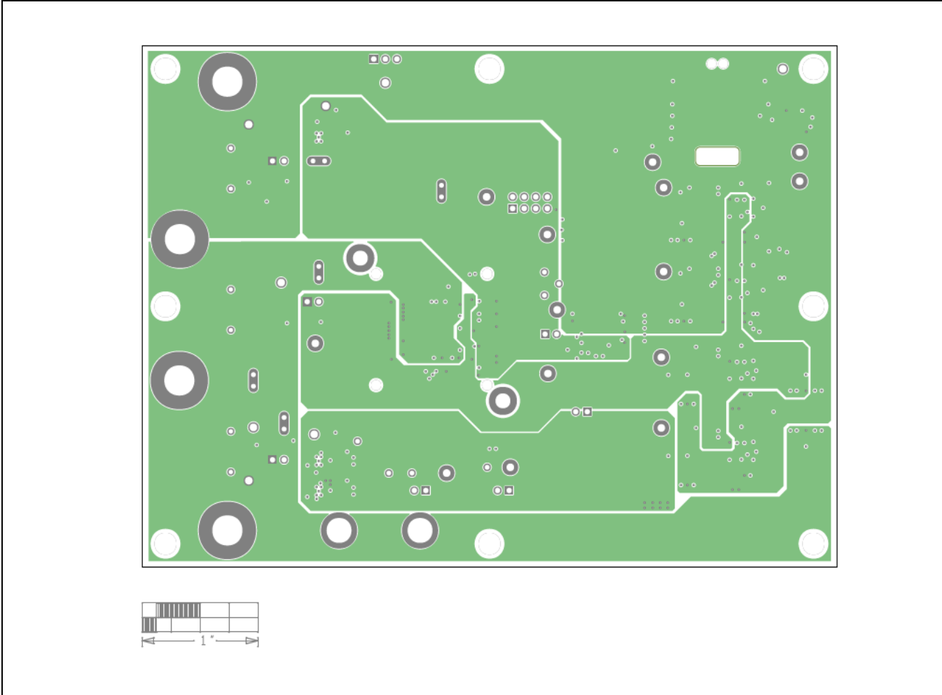
MAX32010 EV Kit PCB Layout—Internal 3
