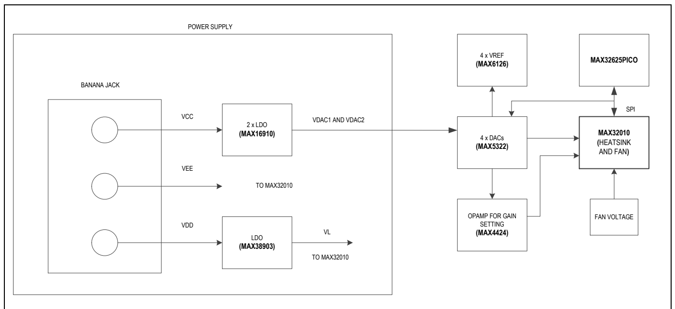
Figure 2. MAX32010 EV Kit Block Diagram
