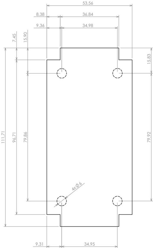
Cover PCB
