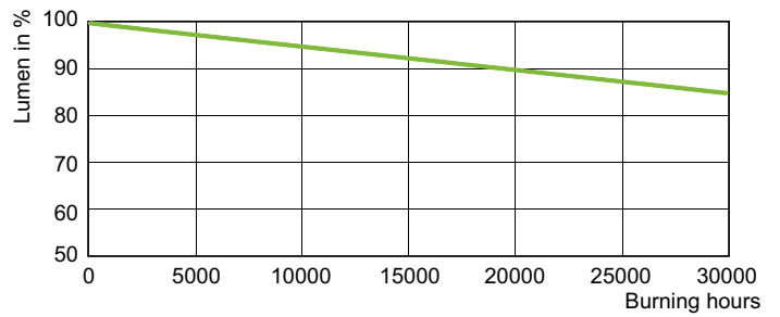
Lumen Maintenance Diagram - SON 400W E E40 CO 1SL/12
