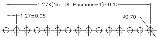
PCB Layout
